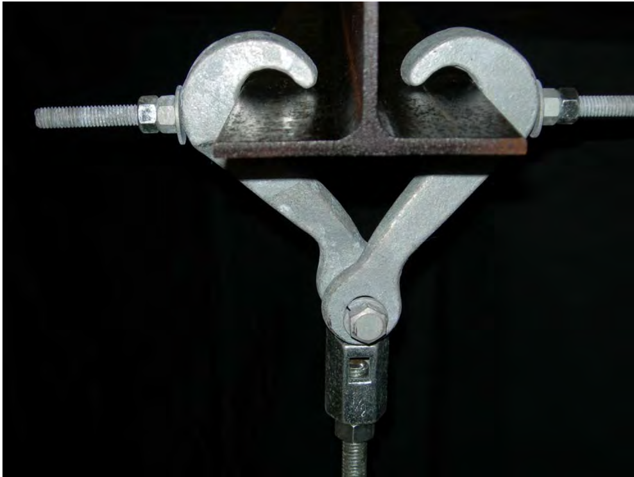
FIG. 232 BEAM CLAMP WITH SWING NUT
