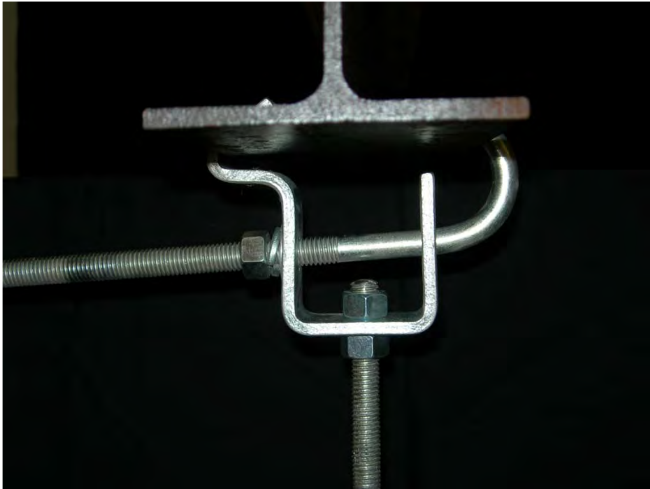
FIG. 38 ADJUSTABLE BEAM CLAMP
